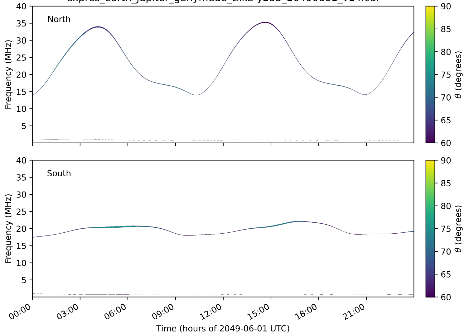
expres_earth_jupiter_ganymede_txka-y235_20490601_v14.cdf
