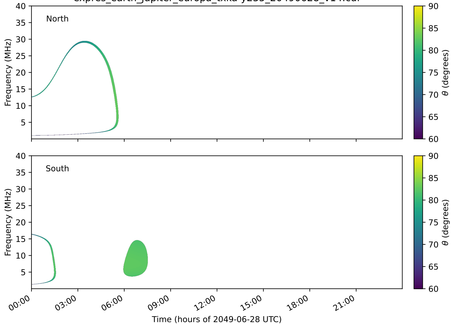
expres_earth_jupiter_europa_txka-y235_20490628_v14.cdf
