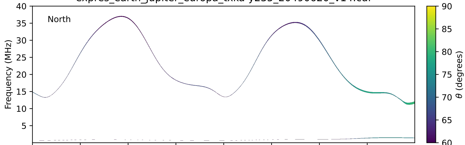
expres_earth_jupiter_europa_txka-y235_20490620_v14.cdf
