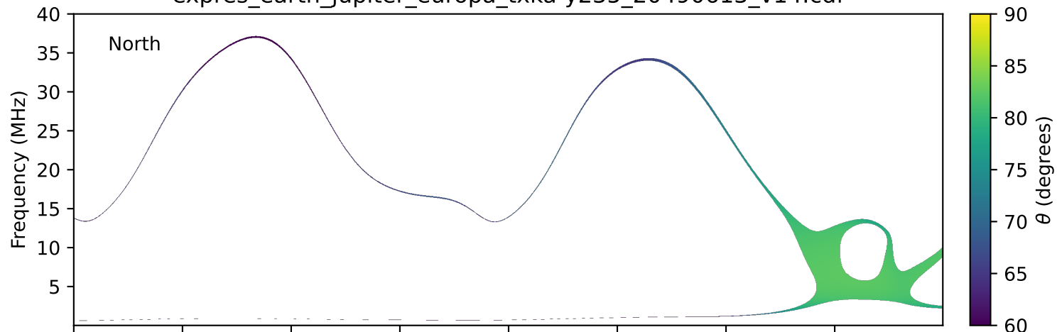
expres_earth_jupiter_europa_txka-y235_20490613_v14.cdf
