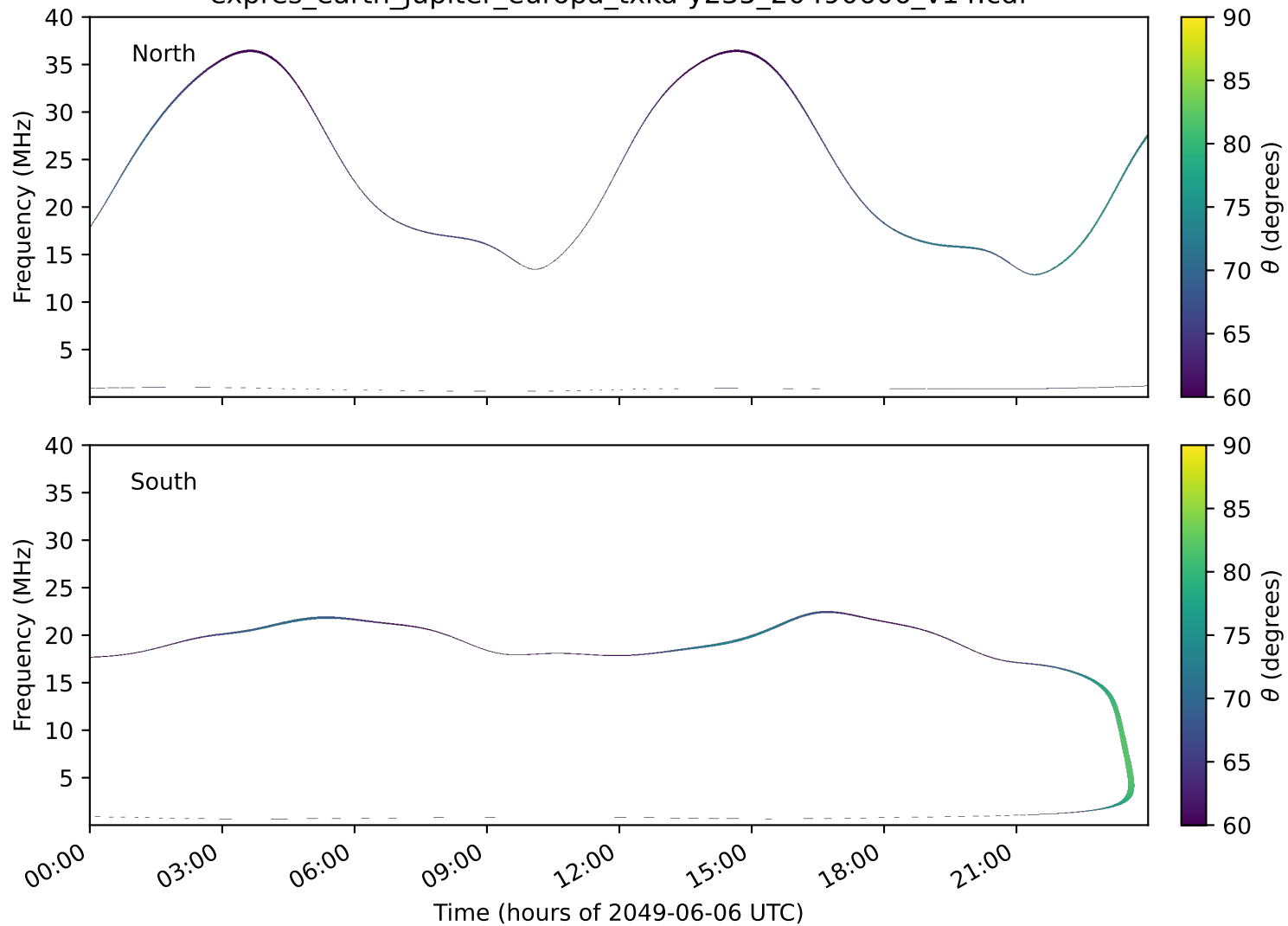
expres_earth_jupiter_europa_txka-y235_20490606_v14.cdf
