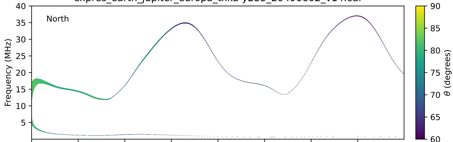
expres_earth_jupiter_europa_txka-y235_20490602_v14.cdf
