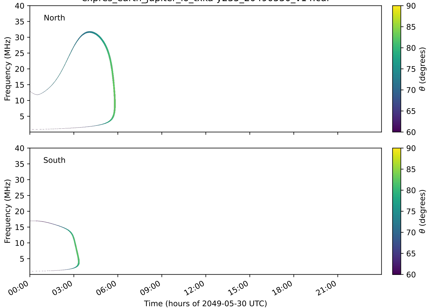
expres_earth_jupiter_io_txka-y235_20490530_v14.cdf
