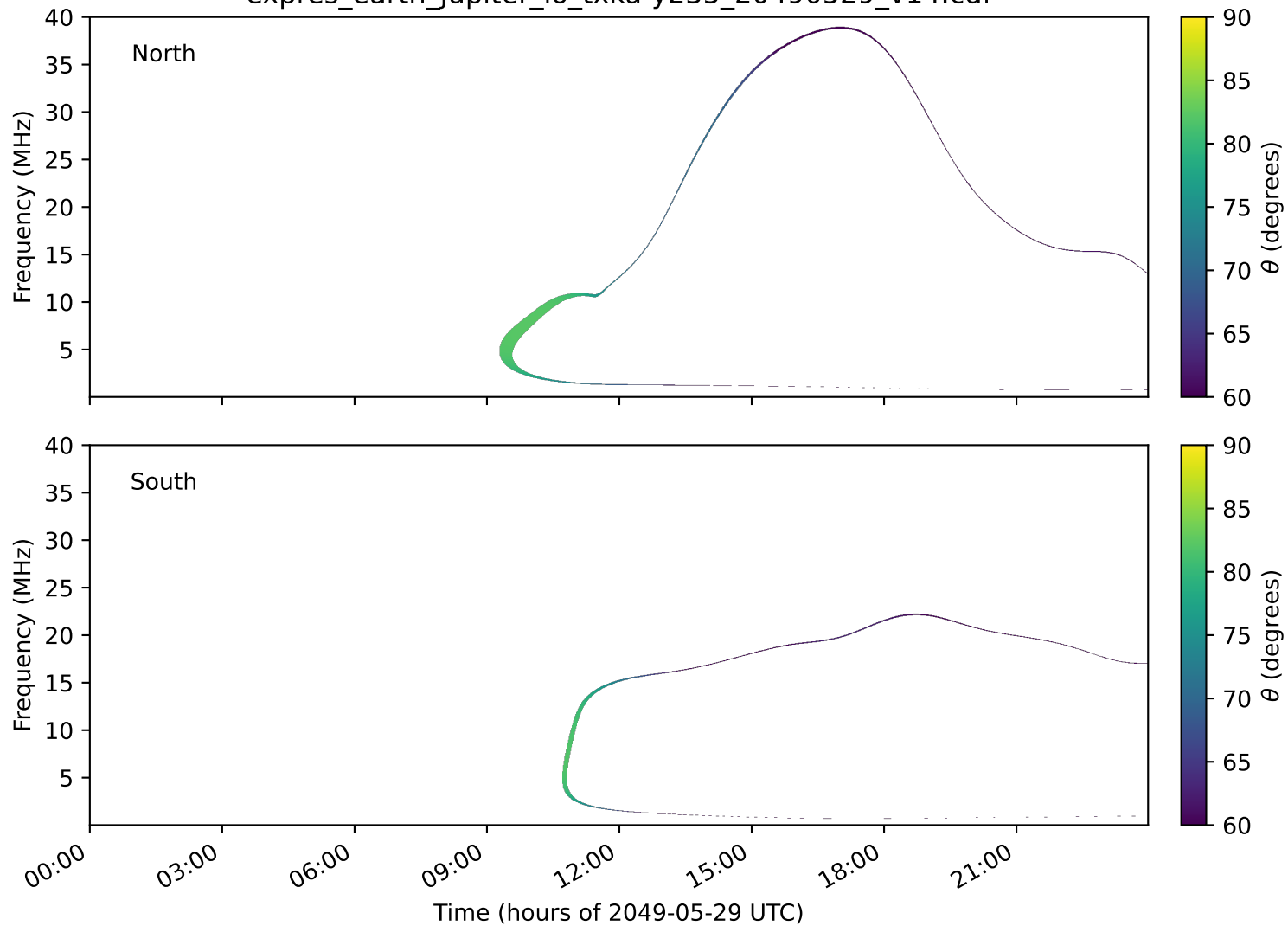
expres_earth_jupiter_io_txka-y235_20490529_v14.cdf
