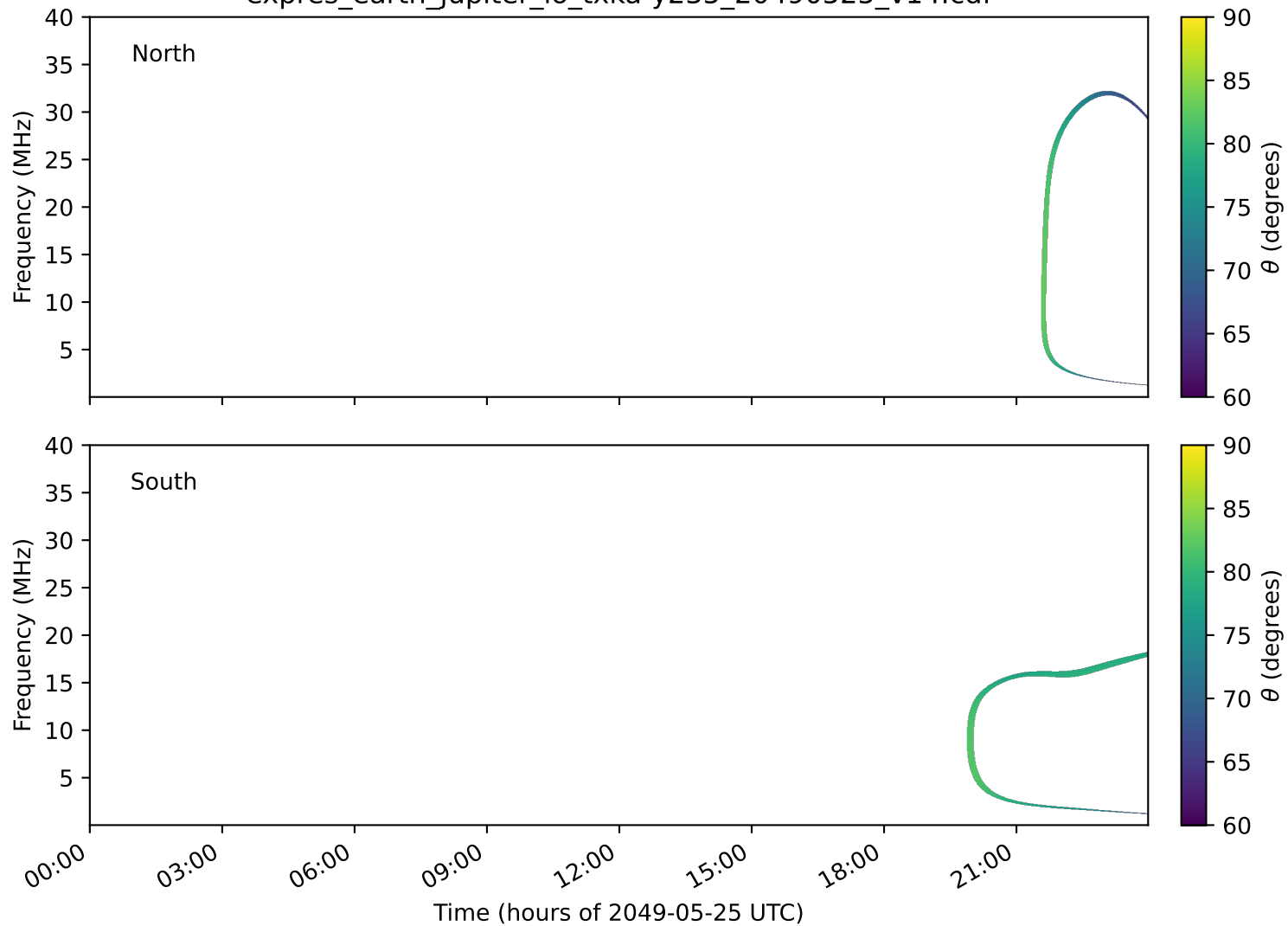
expres_earth_jupiter_io_txka-y235_20490525_v14.cdf
