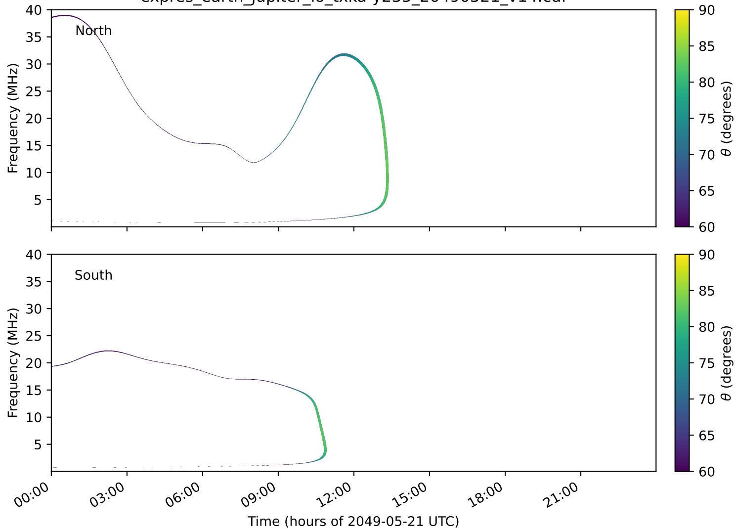
expres_earth_jupiter_io_txka-y235_20490521_v14.cdf
