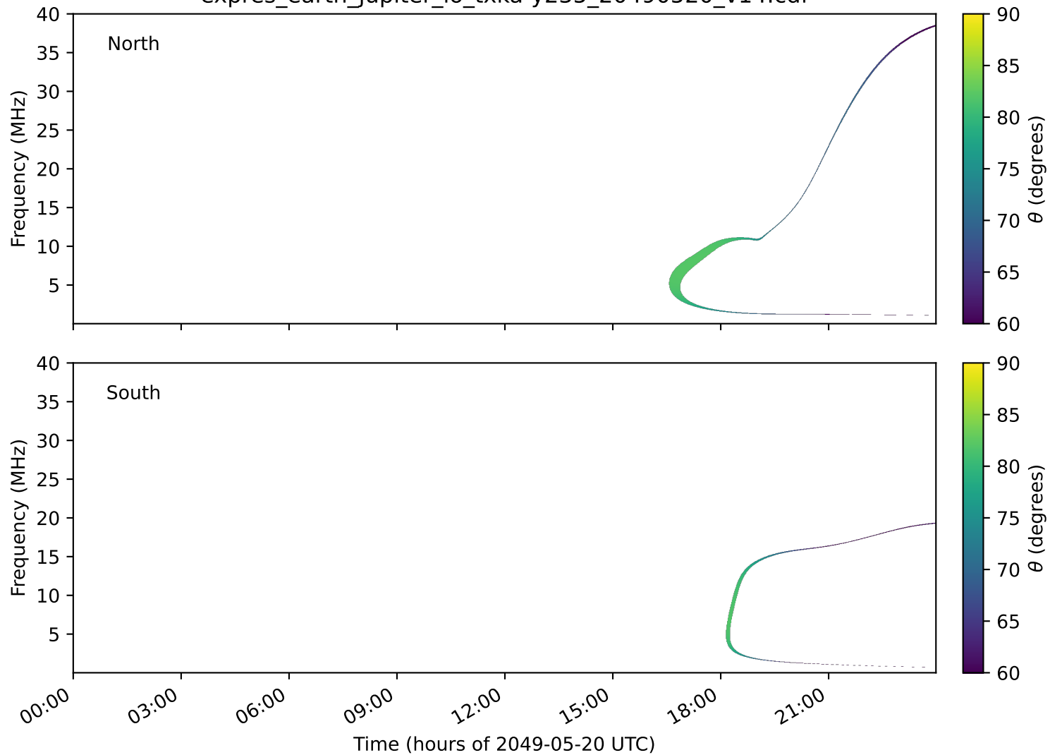
expres_earth_jupiter_io_txka-y235_20490520_v14.cdf
