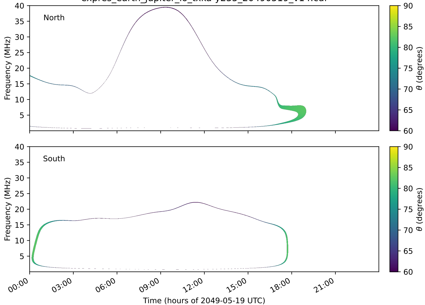
expres_earth_jupiter_io_txka-y235_20490519_v14.cdf
