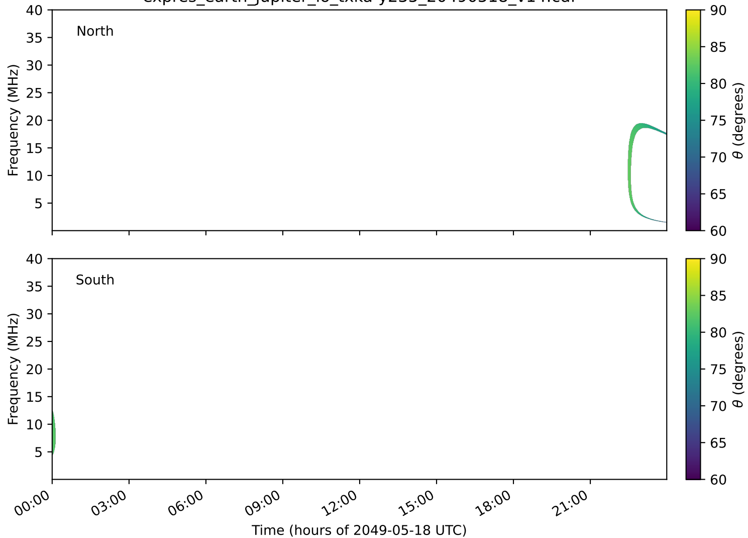
expres_earth_jupiter_io_txka-y235_20490518_v14.cdf
