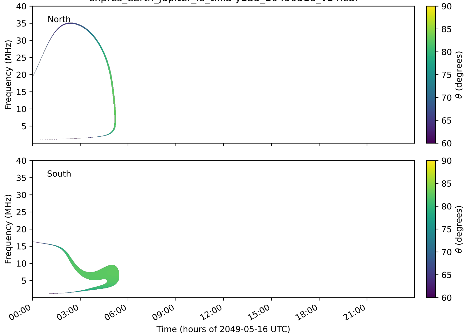
expres_earth_jupiter_io_txka-y235_20490516_v14.cdf
