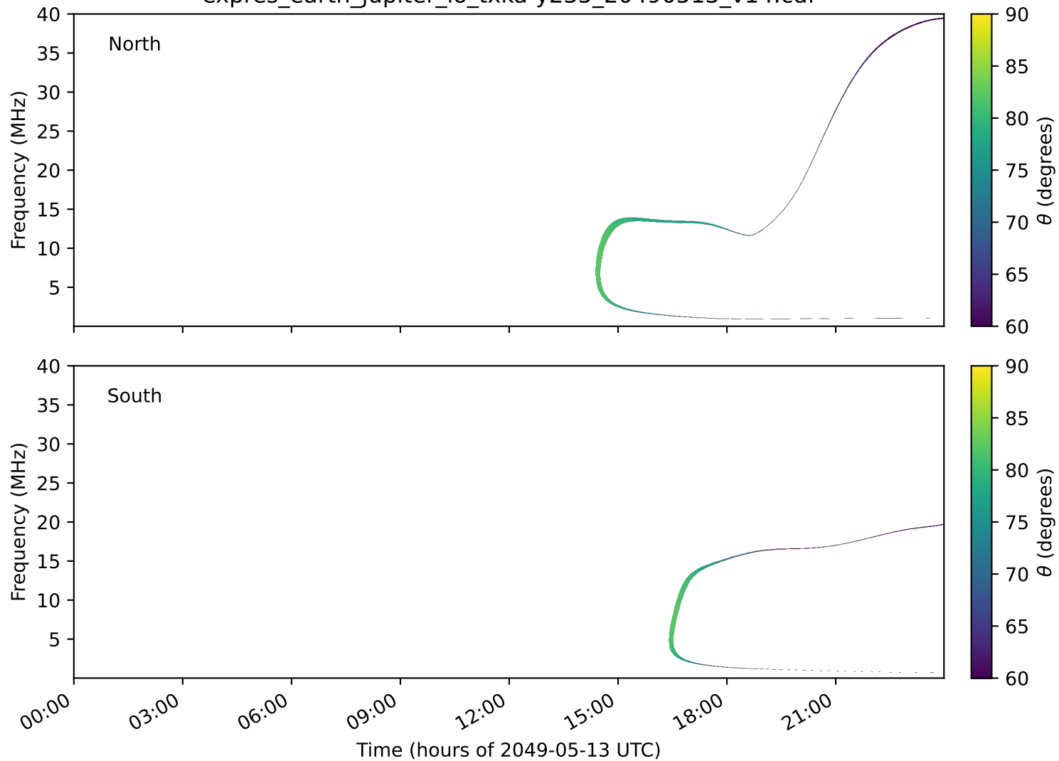
expres_earth_jupiter_io_txka-y235_20490513_v14.cdf
