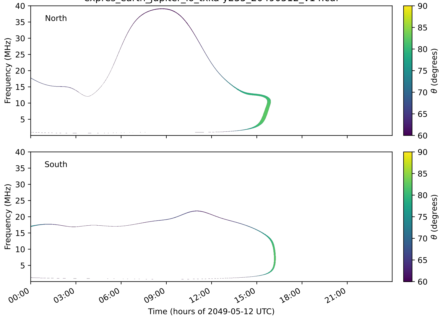
expres_earth_jupiter_io_txka-y235_20490512_v14.cdf
