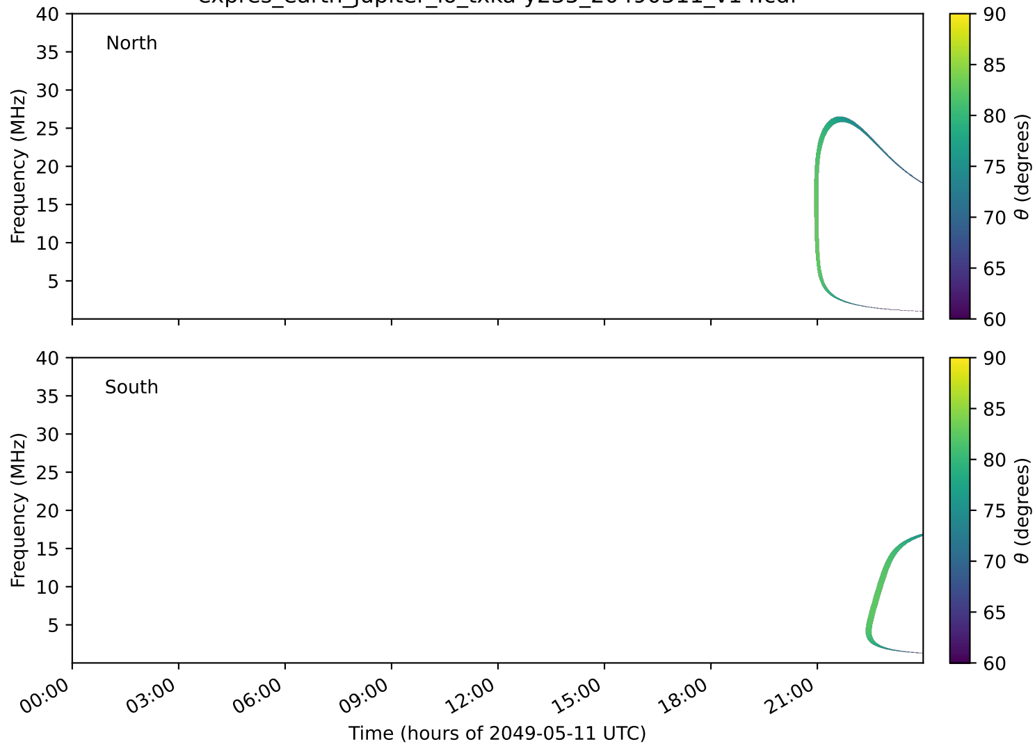
expres_earth_jupiter_io_txka-y235_20490511_v14.cdf
