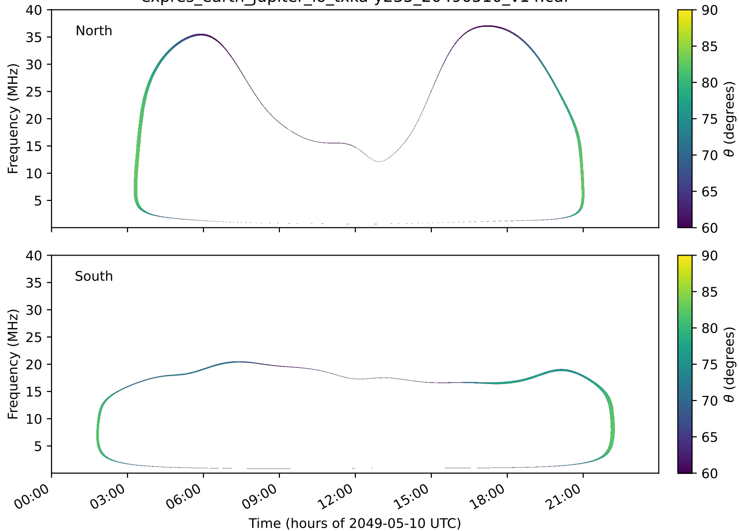
expres_earth_jupiter_io_txka-y235_20490510_v14.cdf
