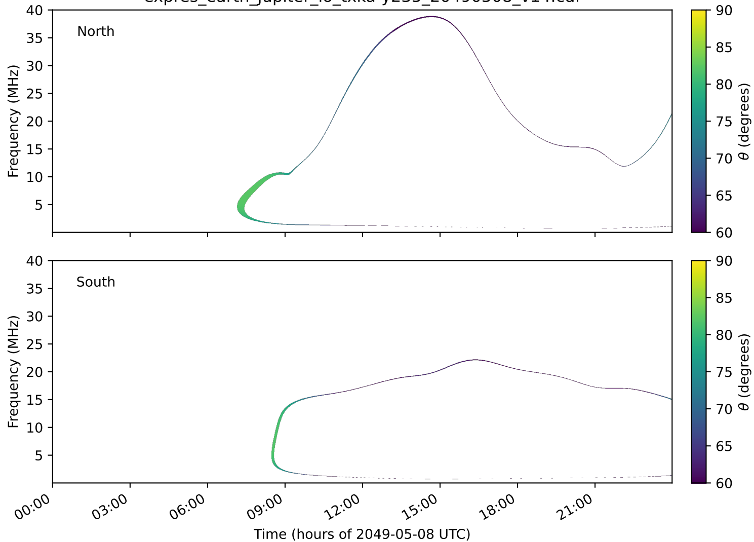
expres_earth_jupiter_io_txka-y235_20490508_v14.cdf
