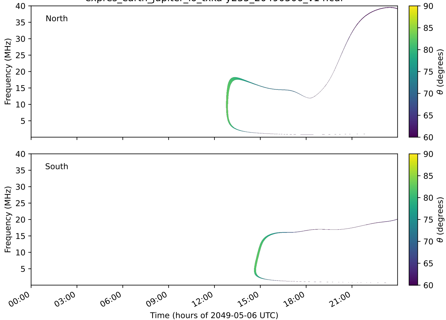
expres_earth_jupiter_io_txka-y235_20490506_v14.cdf
