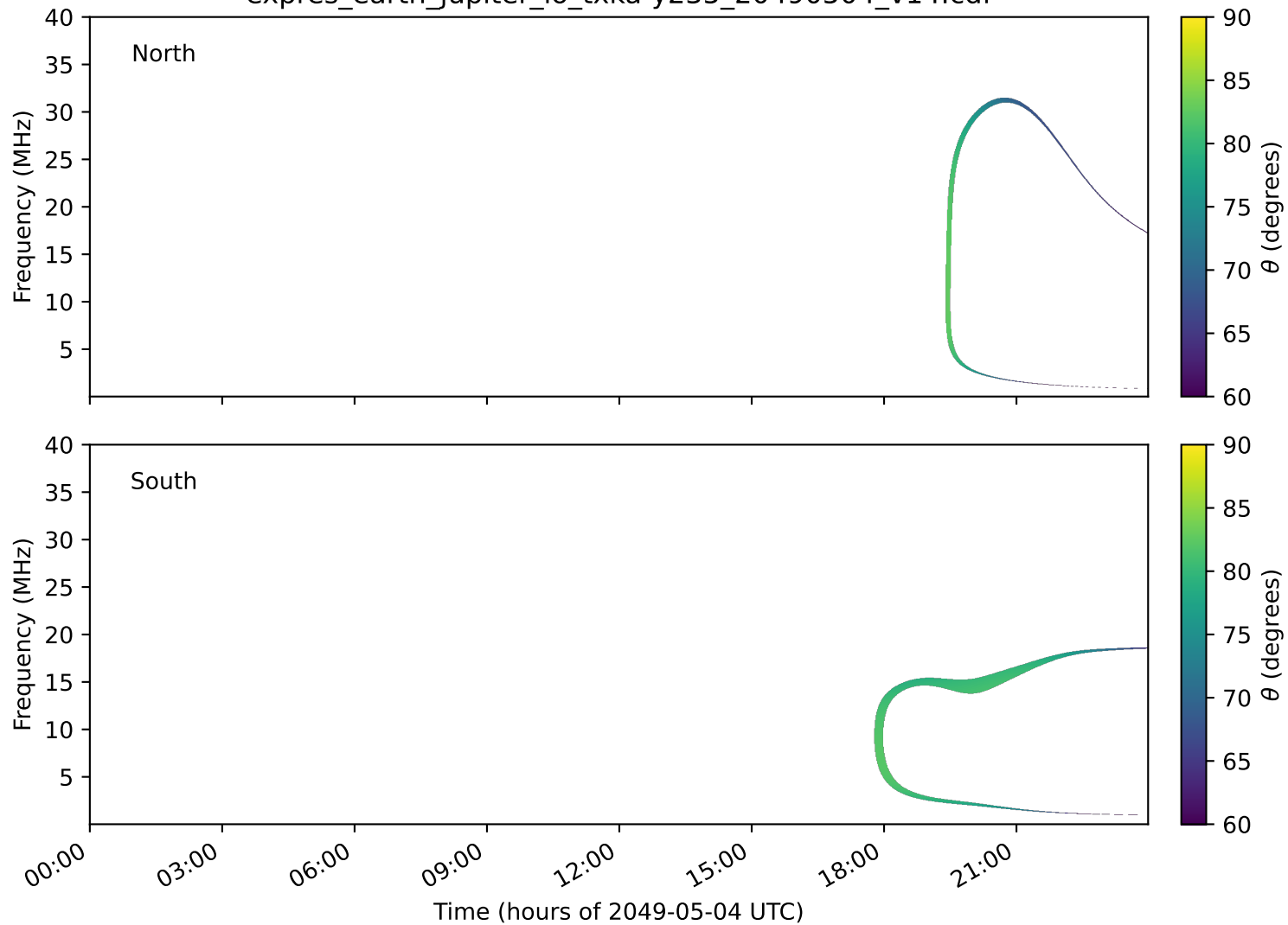
expres_earth_jupiter_io_txka-y235_20490504_v14.cdf
