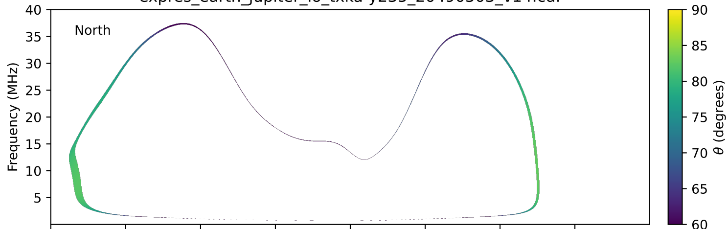
expres_earth_jupiter_io_txka-y235_20490503_v14.cdf
