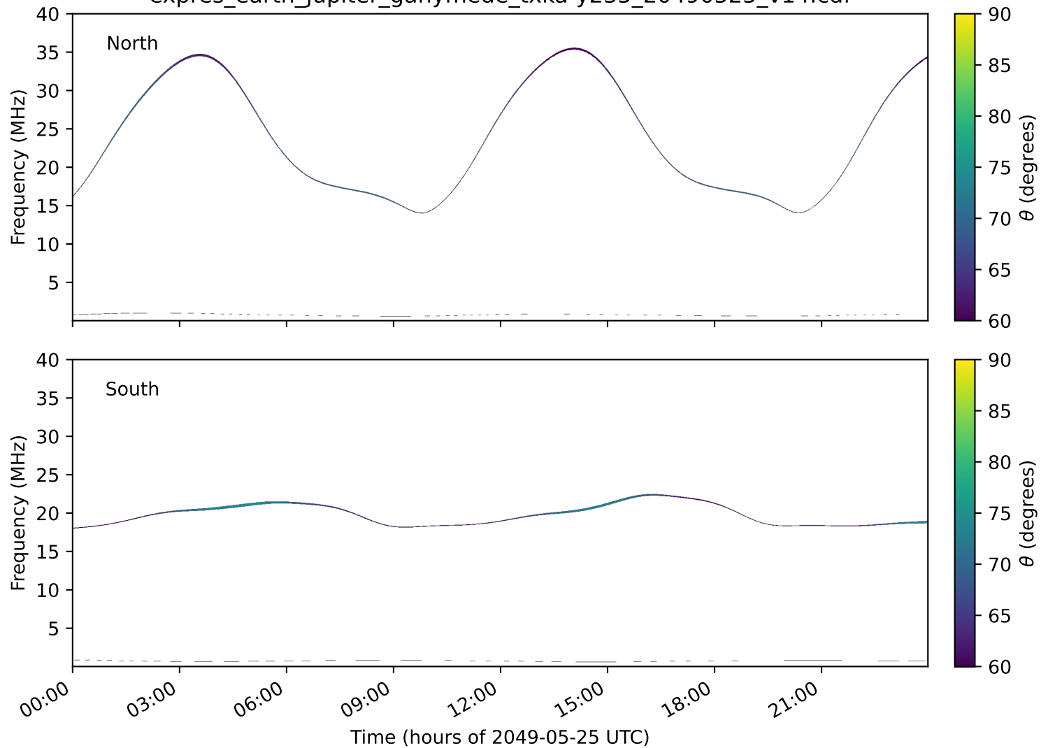
expres_earth_jupiter_ganymede_txka-y235_20490525_v14.cdf
