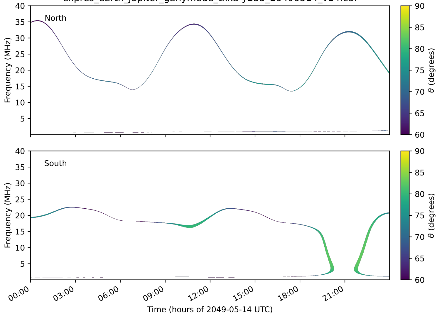
expres_earth_jupiter_ganymede_txka-y235_20490514_v14.cdf
