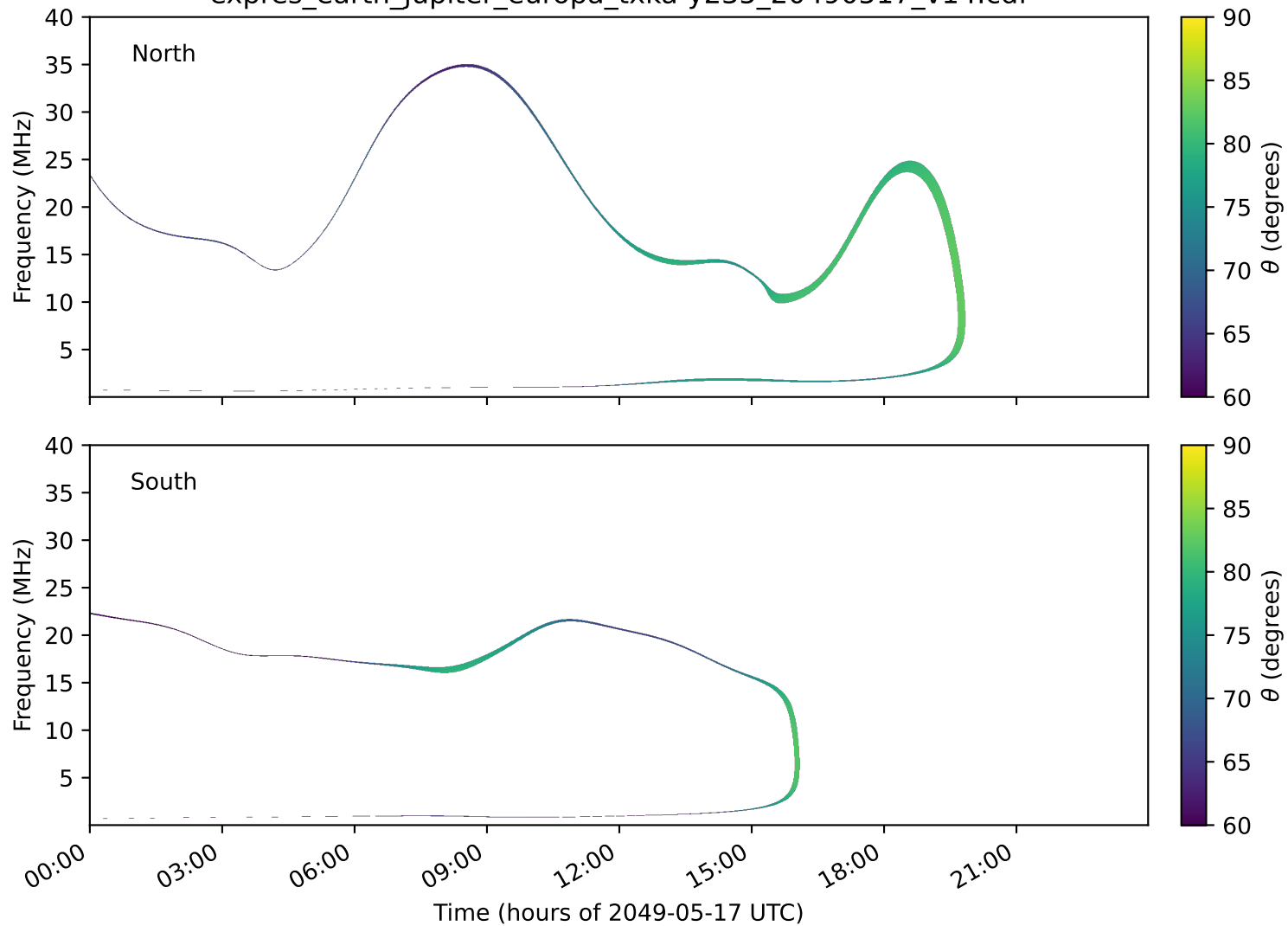
expres_earth_jupiter_europa_txka-y235_20490517_v14.cdf
