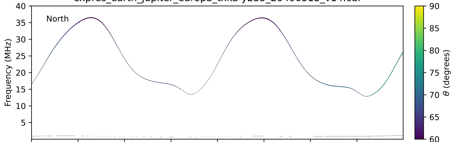
expres_earth_jupiter_europa_txka-y235_20490513_v14.cdf
