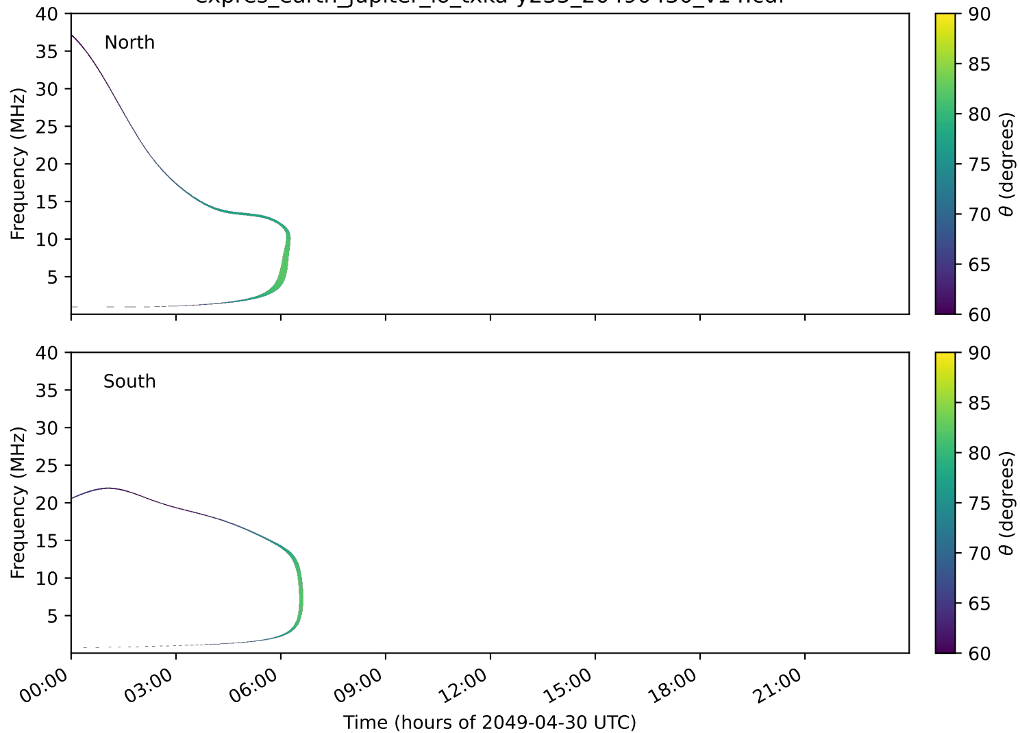
expres_earth_jupiter_io_txka-y235_20490430_v14.cdf
