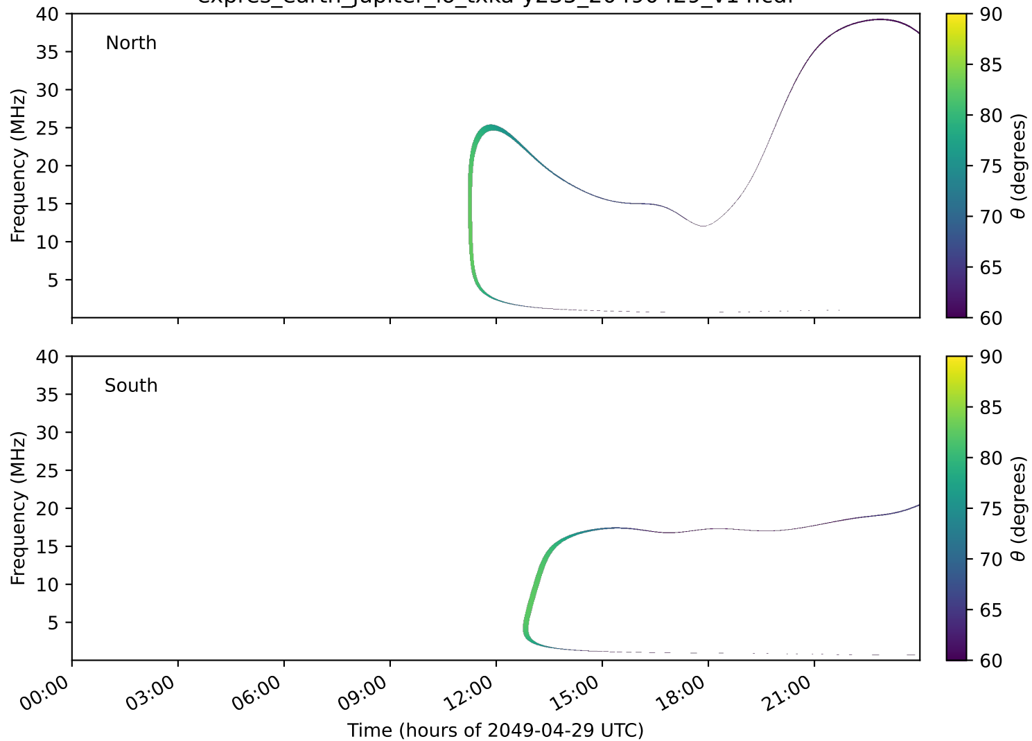
expres_earth_jupiter_io_txka-y235_20490429_v14.cdf
