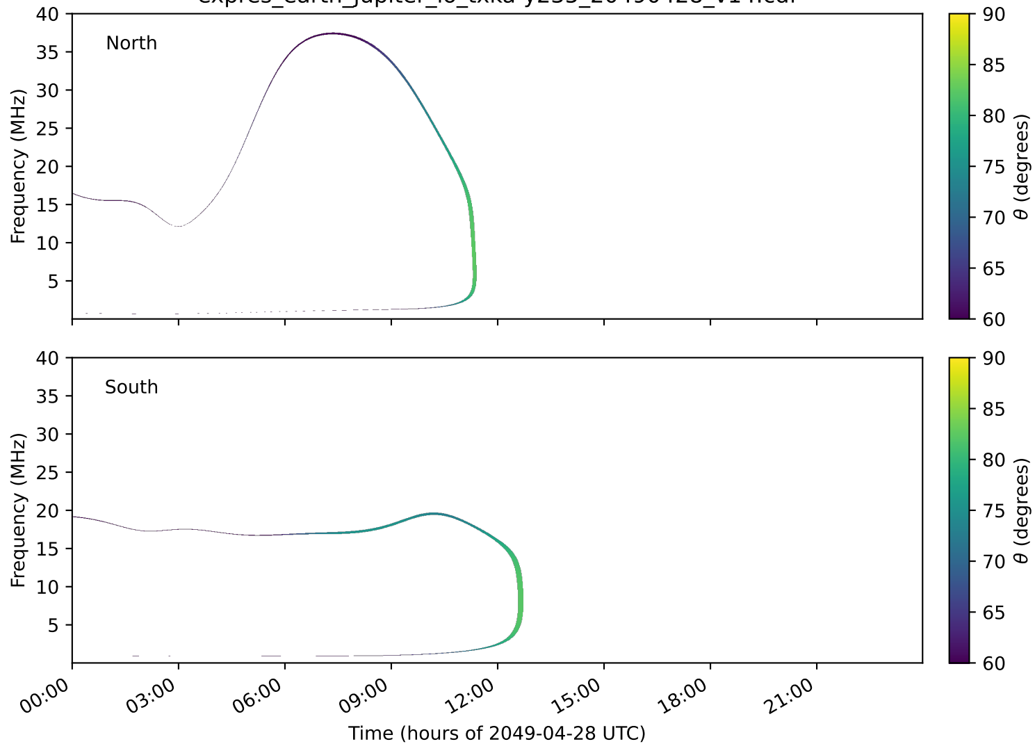
expres_earth_jupiter_io_txka-y235_20490428_v14.cdf
