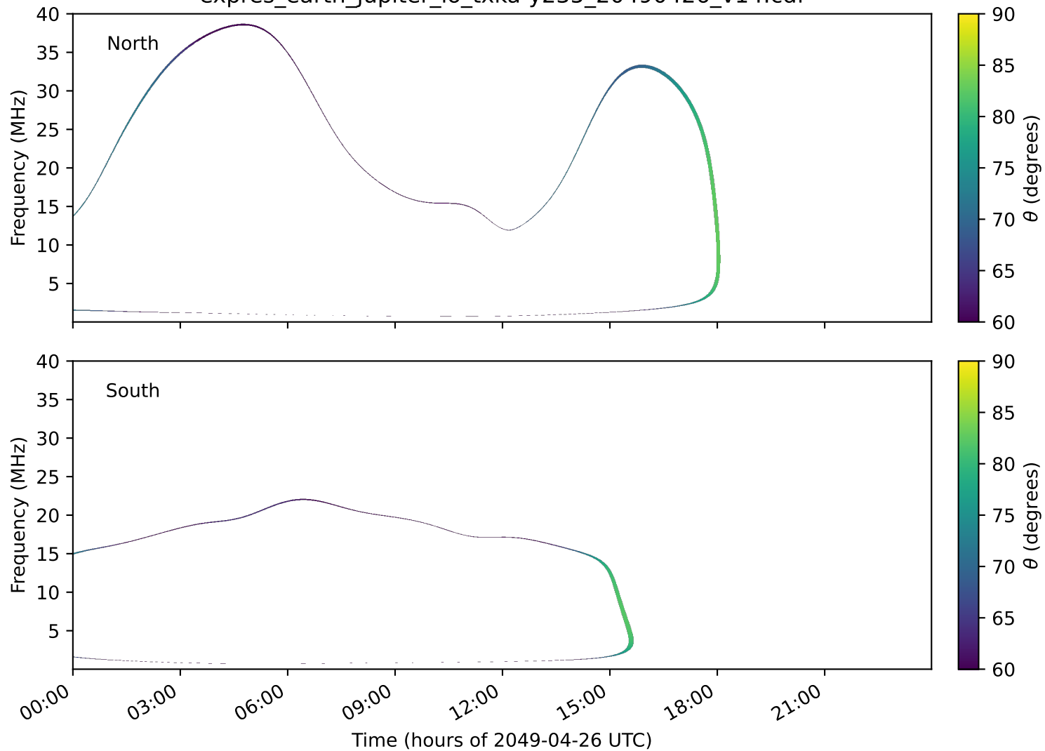
expres_earth_jupiter_io_txka-y235_20490426_v14.cdf
