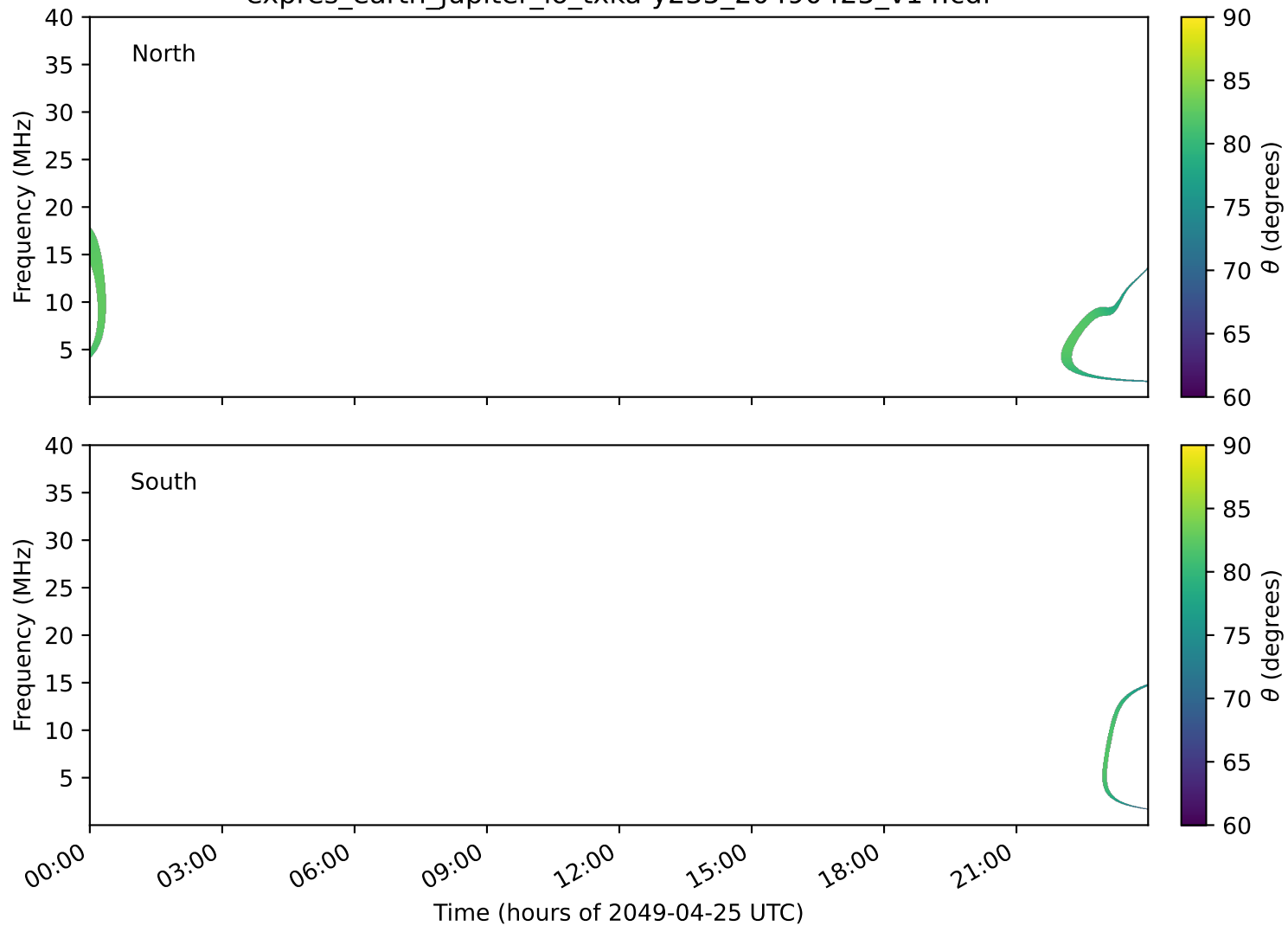
expres_earth_jupiter_io_txka-y235_20490425_v14.cdf
