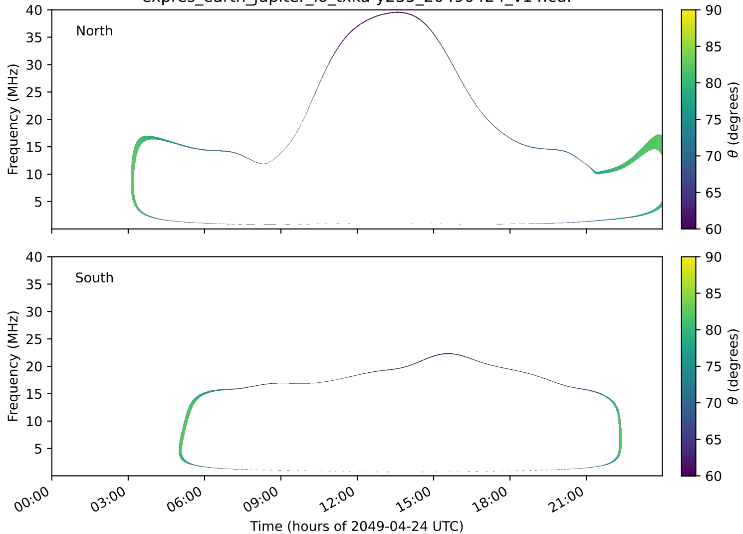
expres_earth_jupiter_io_txka-y235_20490424_v14.cdf
