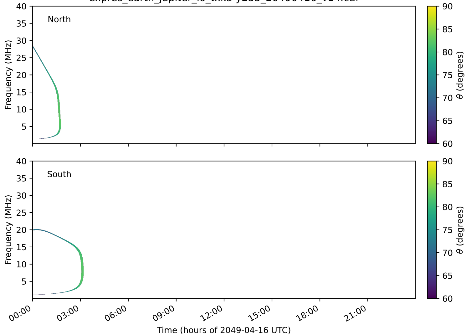
expres_earth_jupiter_io_txka-y235_20490416_v14.cdf
