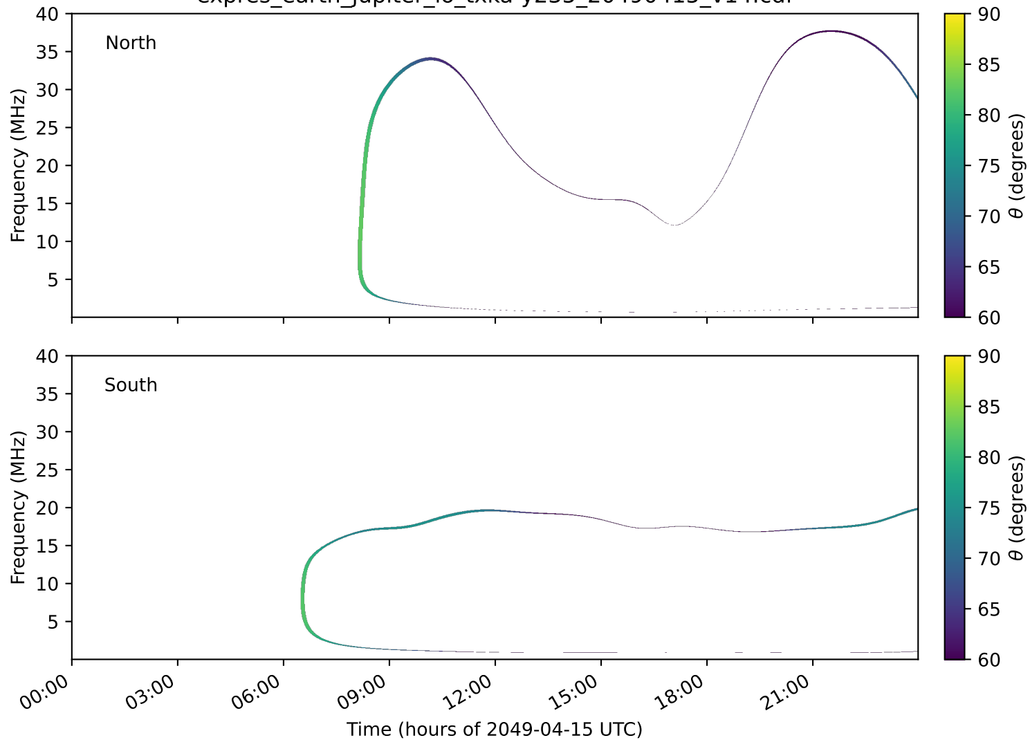
expres_earth_jupiter_io_txka-y235_20490415_v14.cdf
