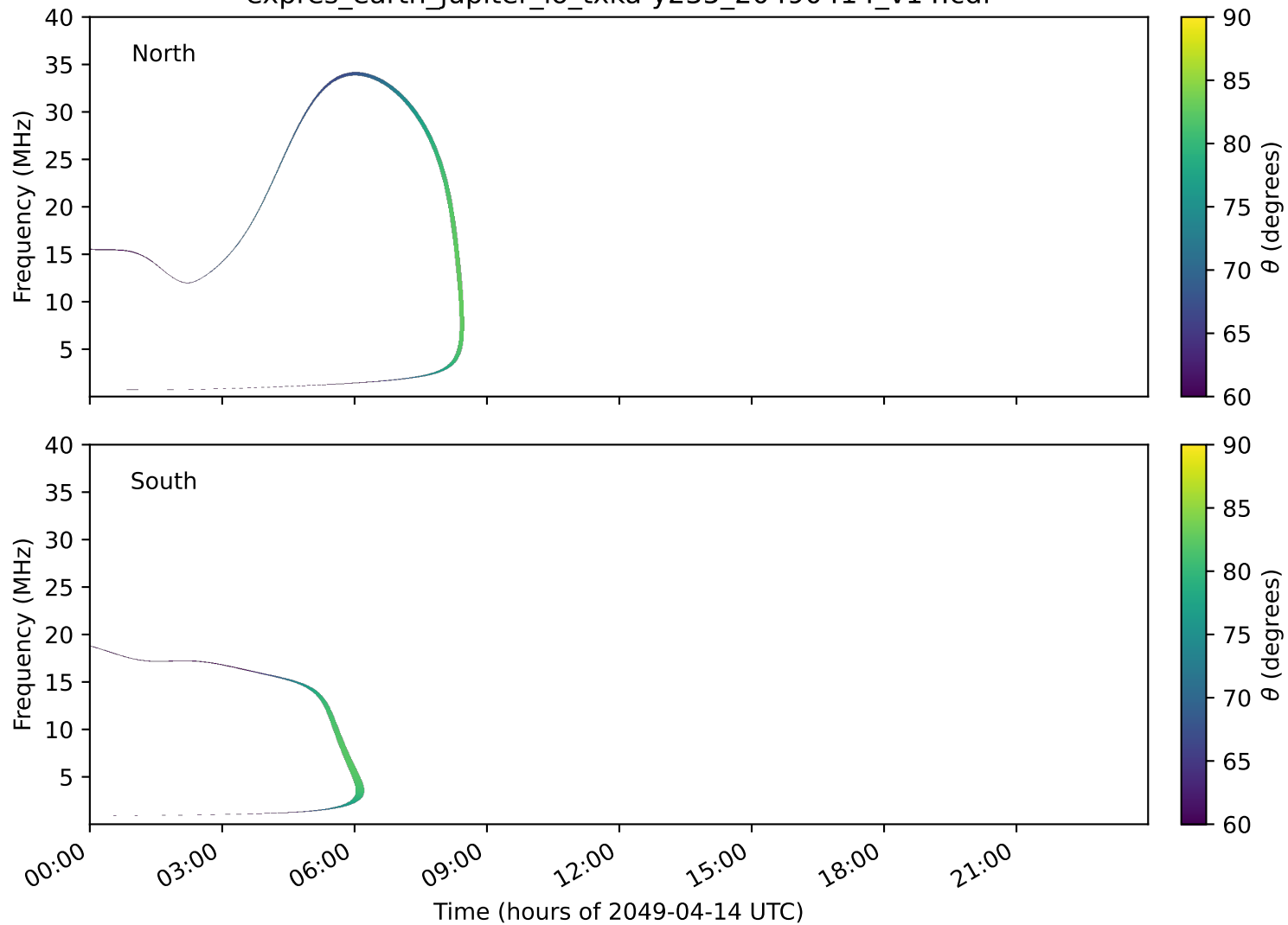
expres_earth_jupiter_io_txka-y235_20490414_v14.cdf
