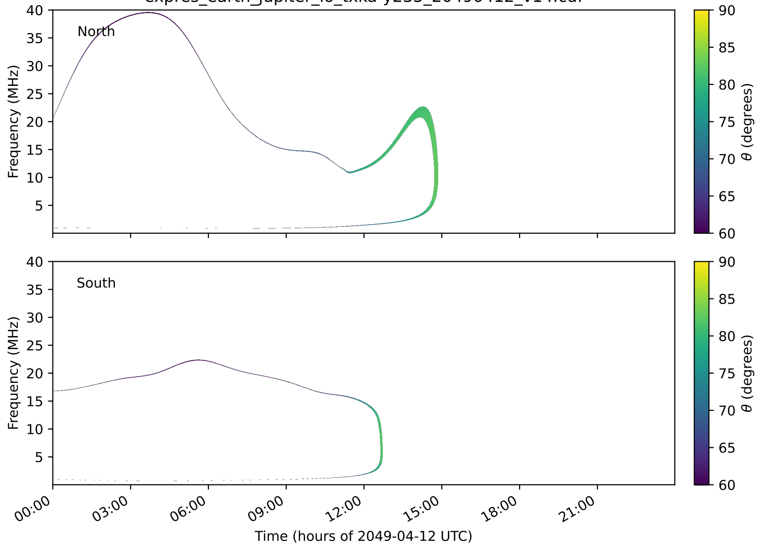
expres_earth_jupiter_io_txka-y235_20490412_v14.cdf
