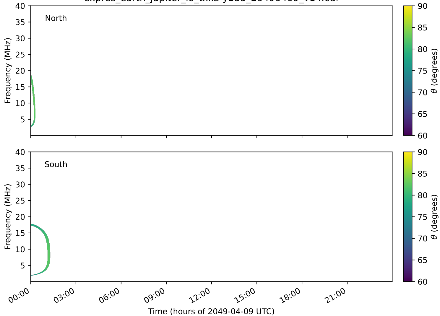
expres_earth_jupiter_io_txka-y235_20490409_v14.cdf
