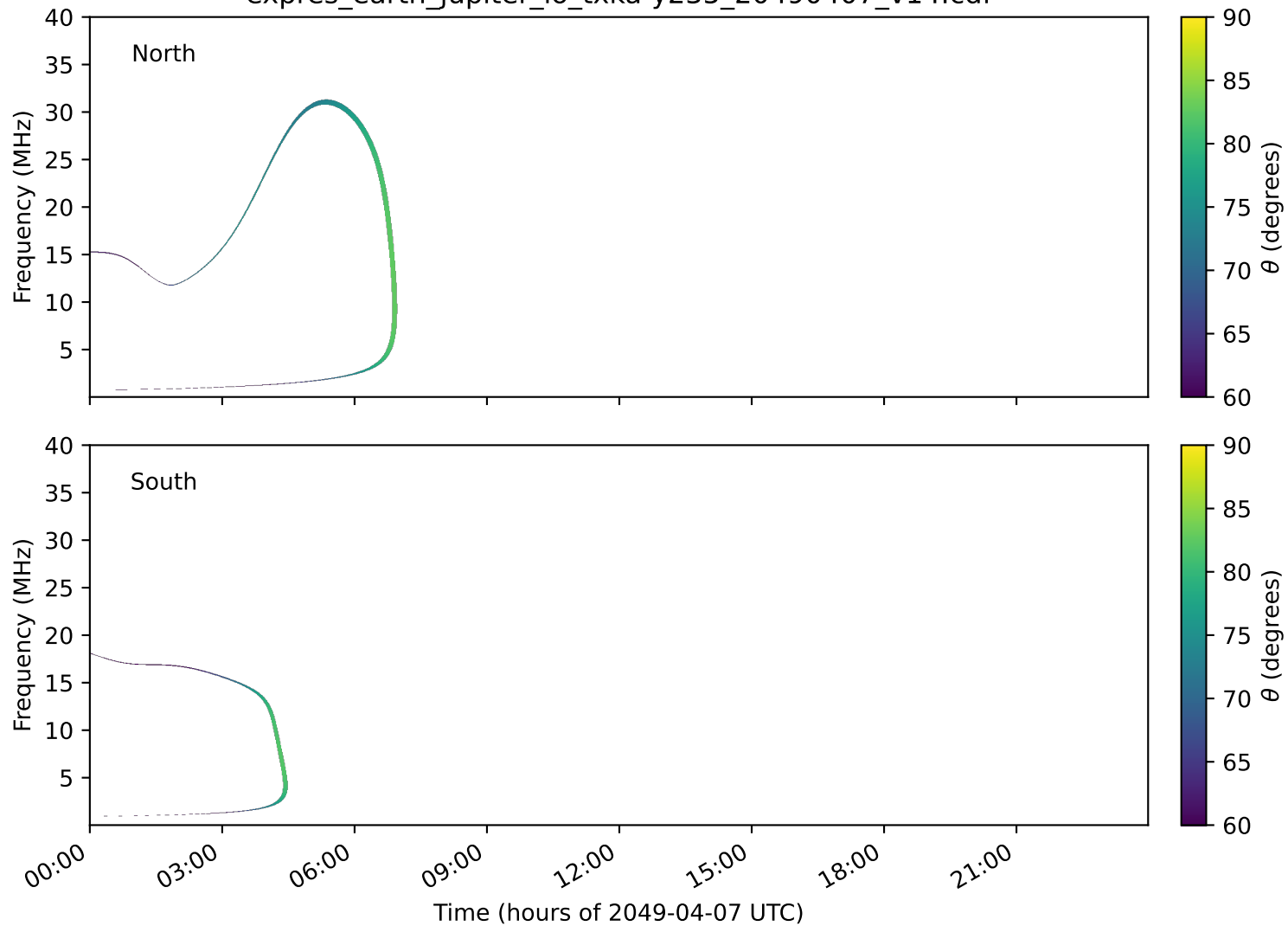
expres_earth_jupiter_io_txka-y235_20490407_v14.cdf
