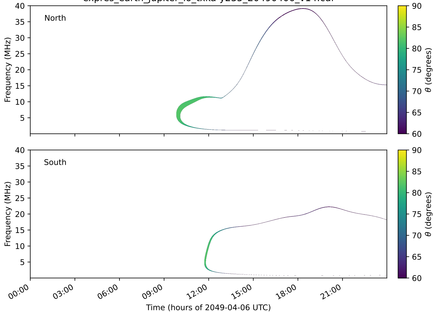
expres_earth_jupiter_io_txka-y235_20490406_v14.cdf
