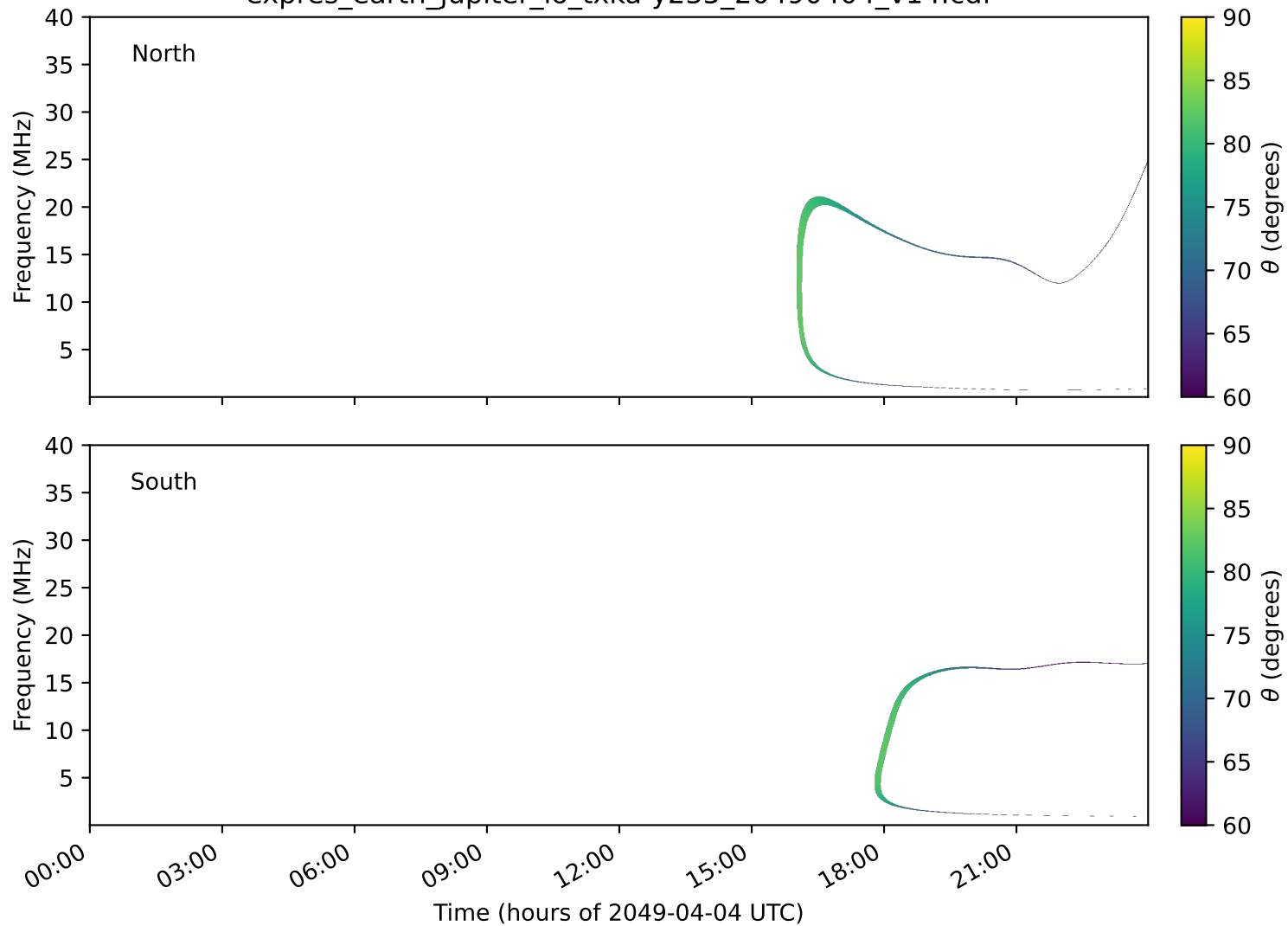
expres_earth_jupiter_io_txka-y235_20490404_v14.cdf
