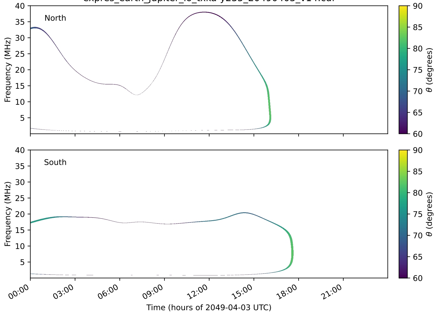
expres_earth_jupiter_io_txka-y235_20490403_v14.cdf
