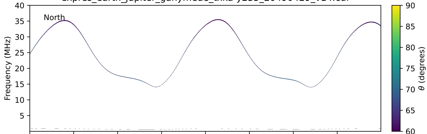
expres_earth_jupiter_ganymede_txka-y235_20490429_v14.cdf
