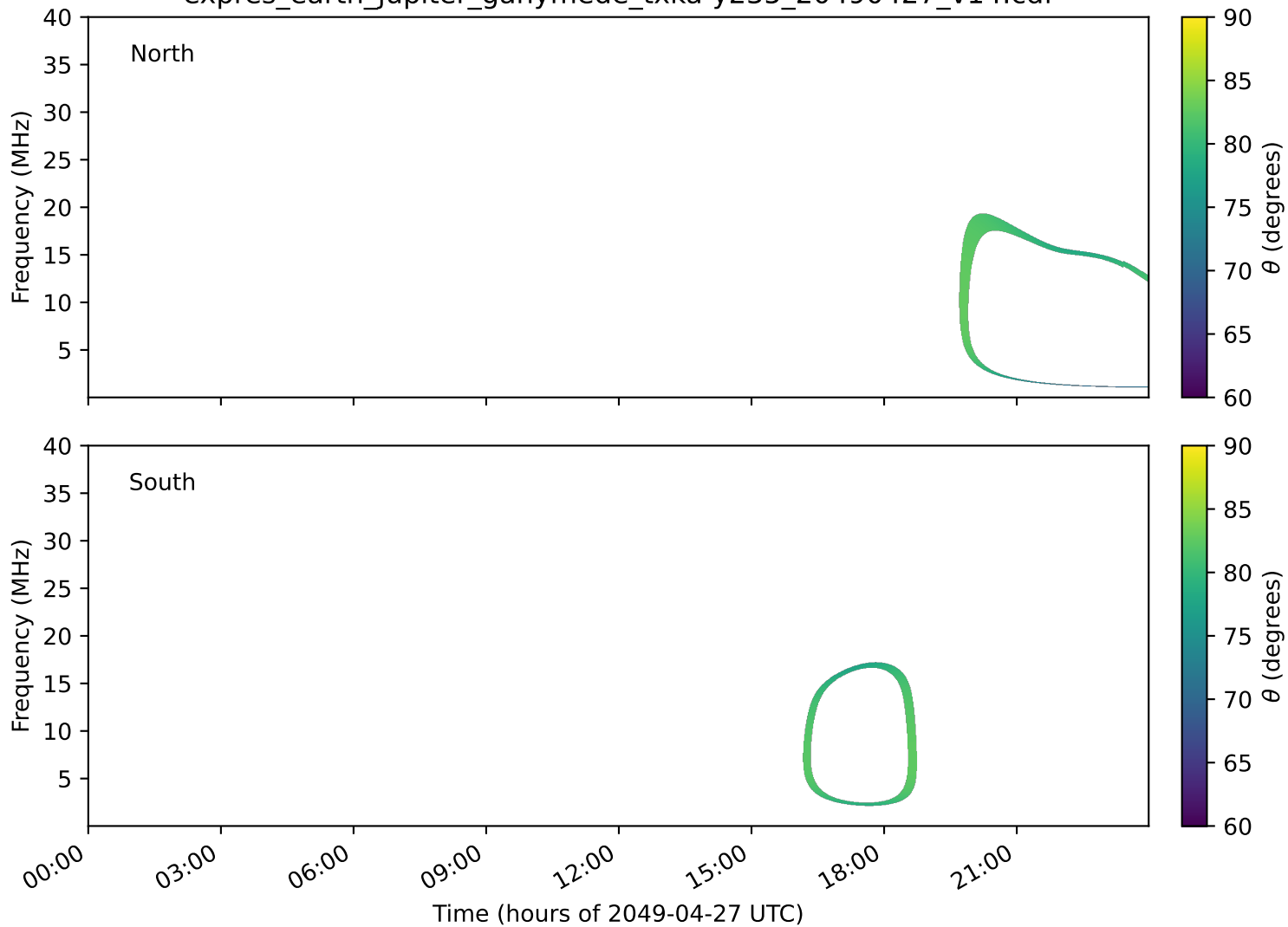
expres_earth_jupiter_ganymede_txka-y235_20490427_v14.cdf
