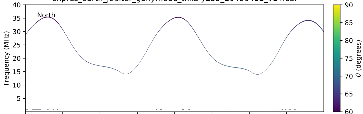
expres_earth_jupiter_ganymede_txka-y235_20490422_v14.cdf
