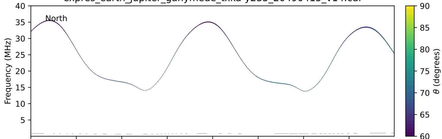
expres_earth_jupiter_ganymede_txka-y235_20490415_v14.cdf
