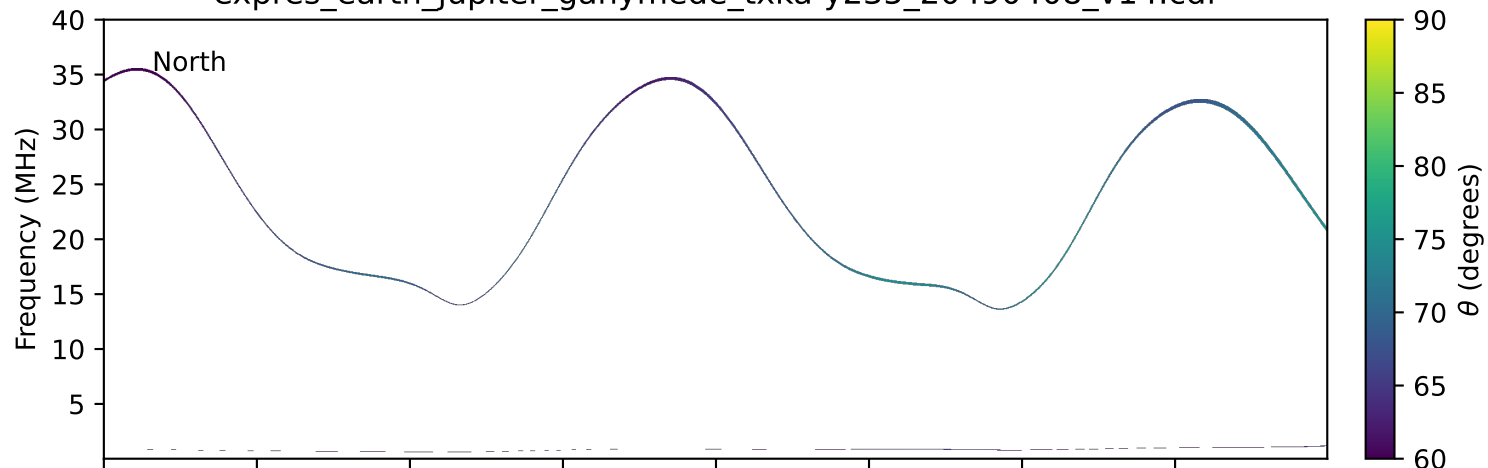
expres_earth_jupiter_ganymede_txka-y235_20490408_v14.cdf
