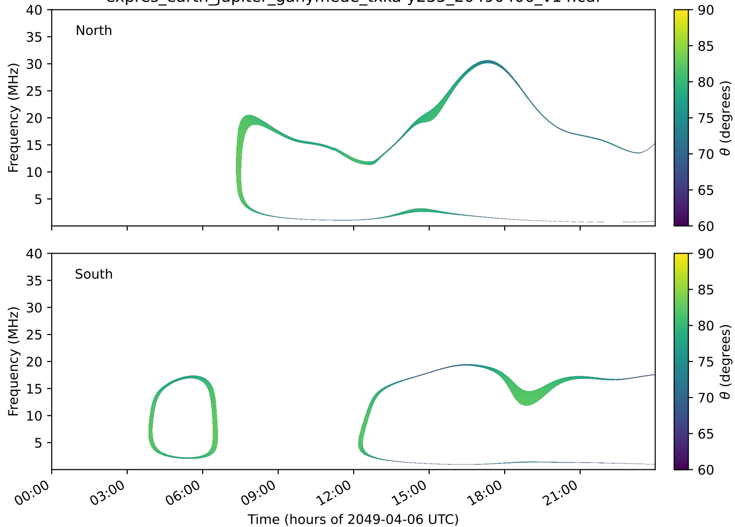
expres_earth_jupiter_ganymede_txka-y235_20490406_v14.cdf
