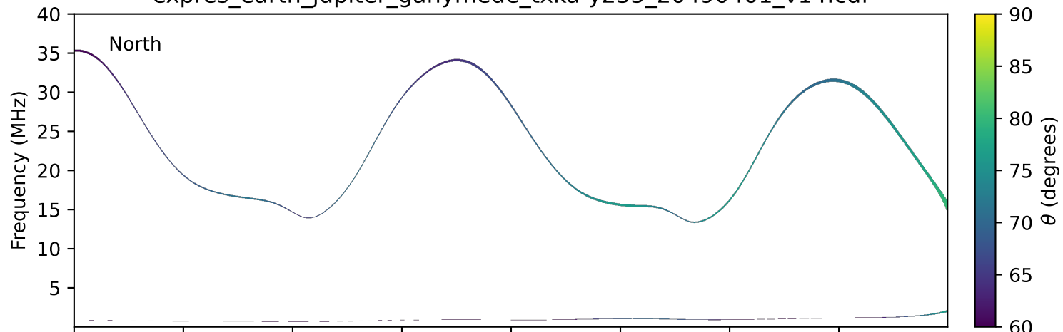
expres_earth_jupiter_ganymede_txka-y235_20490401_v14.cdf
