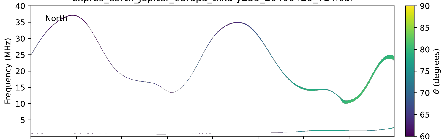
expres_earth_jupiter_europa_txka-y235_20490429_v14.cdf
