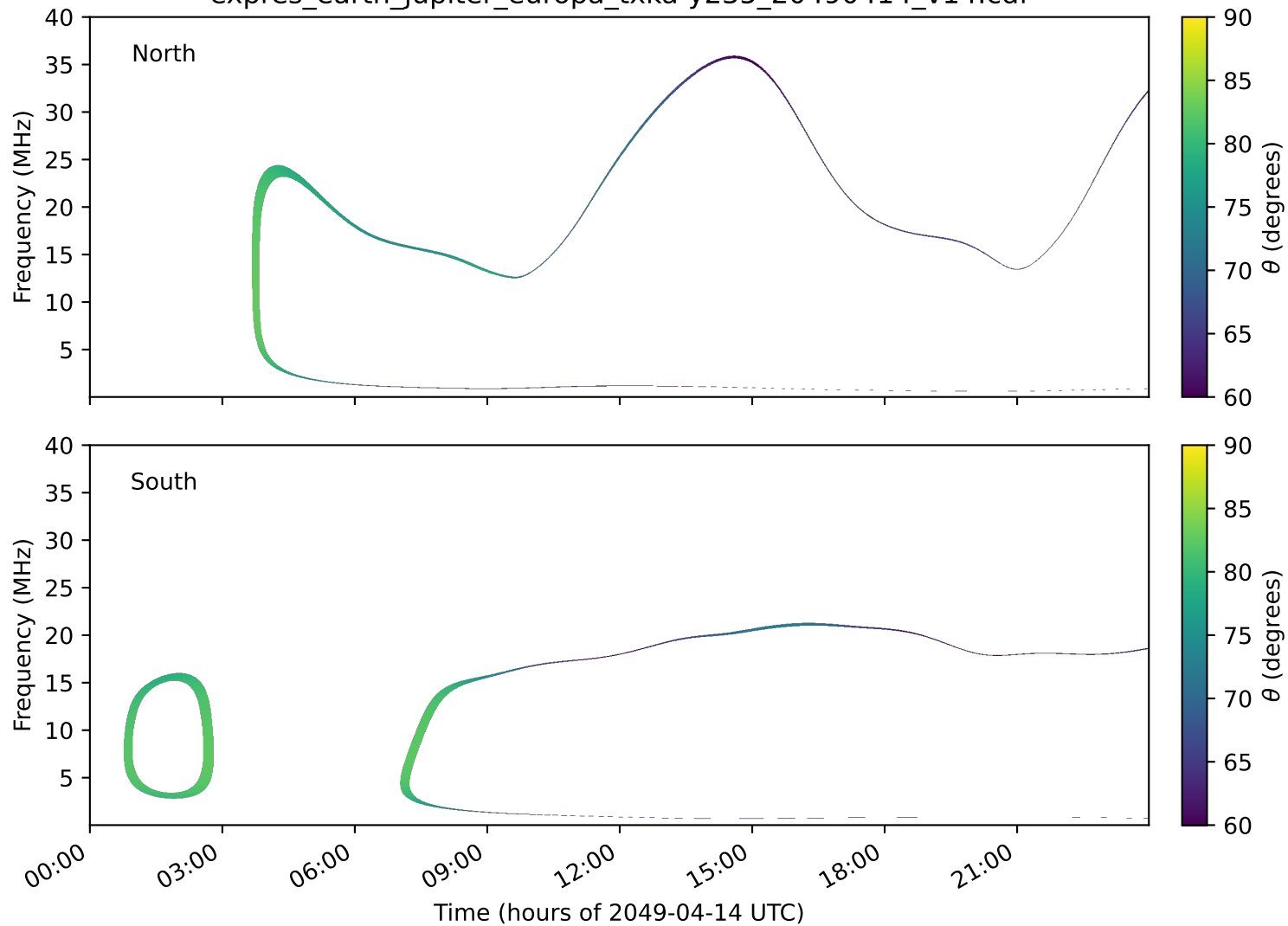
expres_earth_jupiter_europa_txka-y235_20490414_v14.cdf
